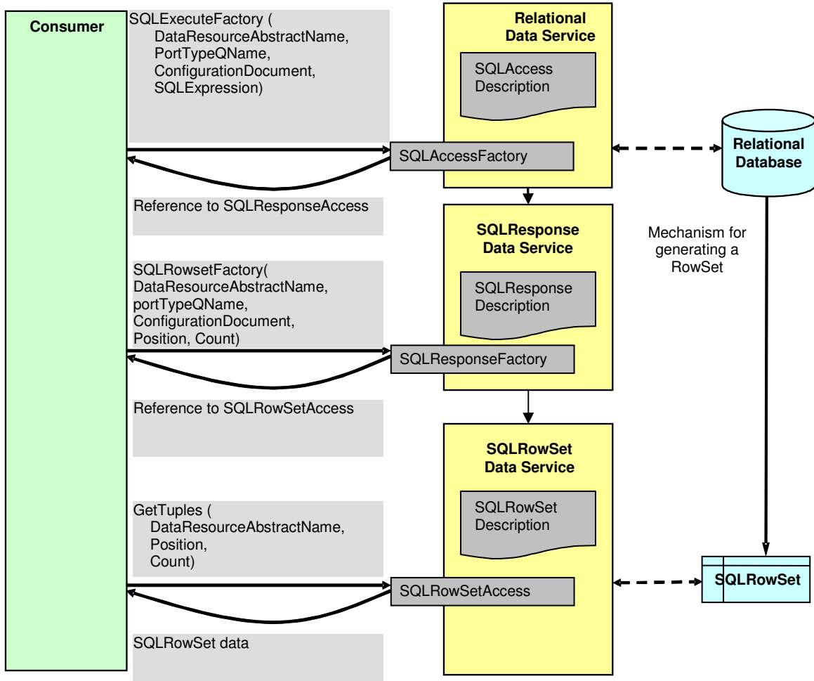
Figure 3 – Overview – SQLResponseFactory
