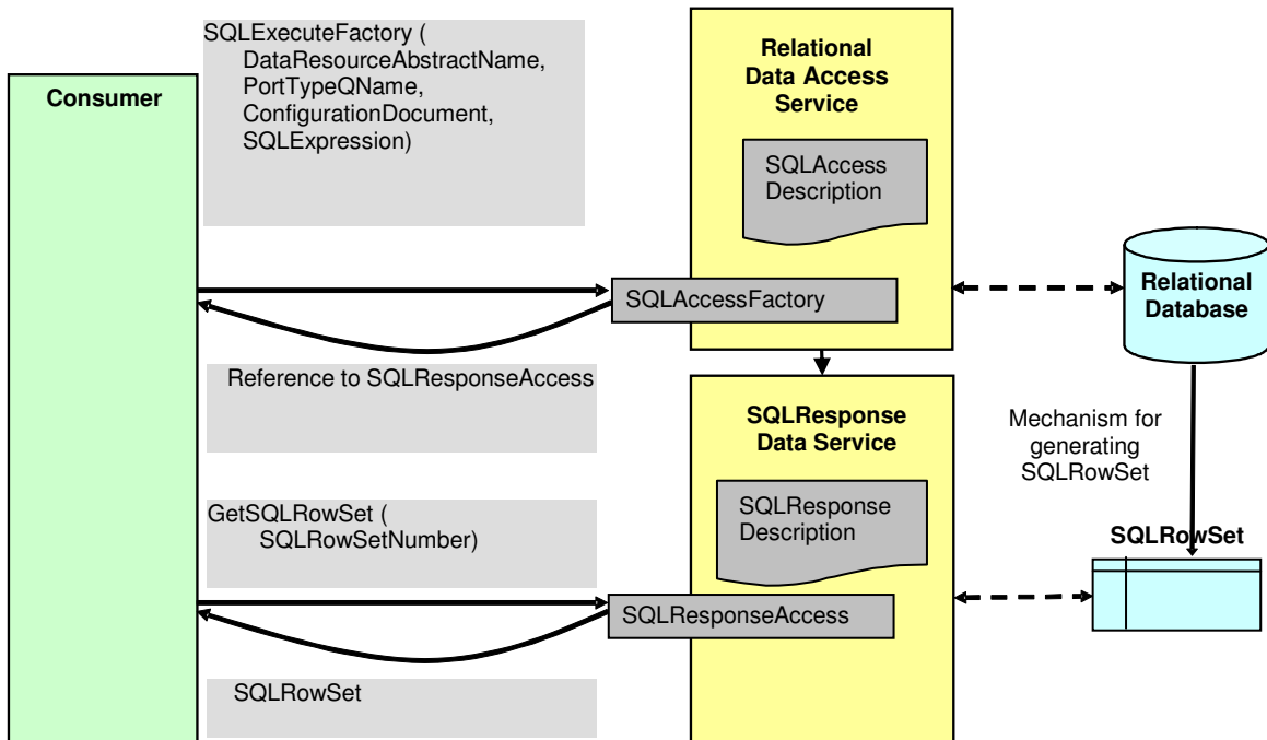
Figure 2 – Overview – SQLAccessFactory
